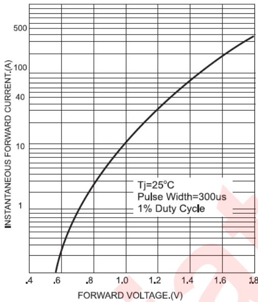
FIG.3-TYPICAL FORWARD CHARACTERISTICS
