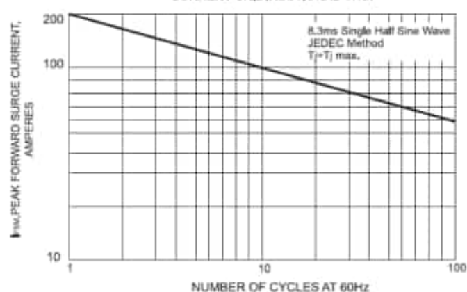
FIG.6-MAXIMUM NON-REPETITIVE FORWARD SURGE CURRENT UNIDIRECTIONAL ONLY
