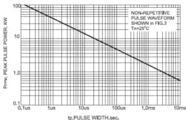
FIG.1-PEAK PULSE POWER RATONG CURRENT
