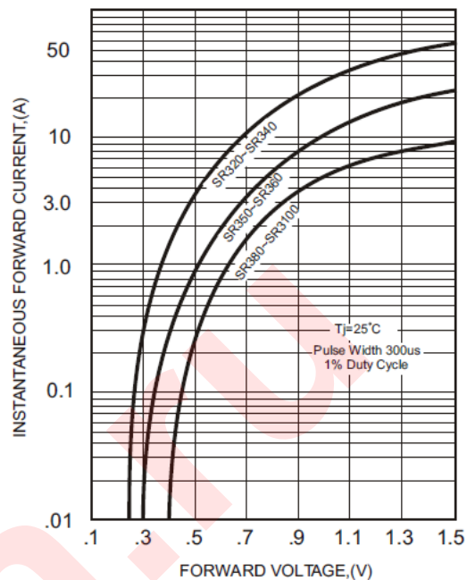
FIG.2-TYPICAL FORWARD CHARACTERISTICS
