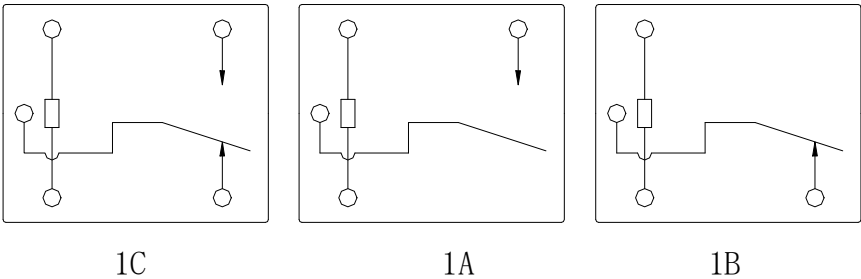
(Bottom View 底视)
