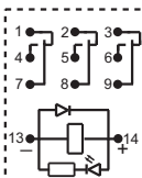
3 Form C (DC, With fly-wheel diode)
