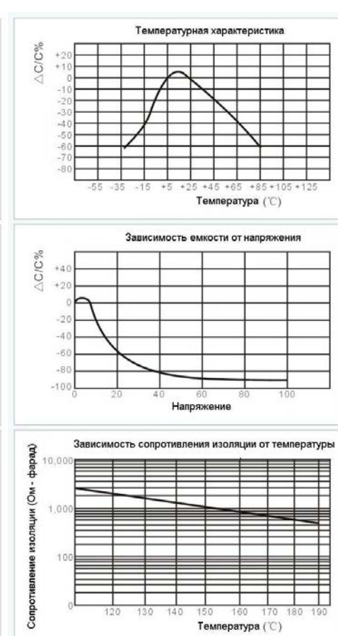
Y5V
