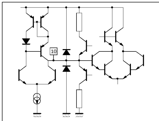
Figure 8 : Pin 10 (SLPF)
