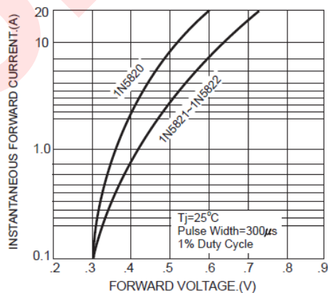
FIG.4-TYPICAL FORWARD CHARACTERISTICS
