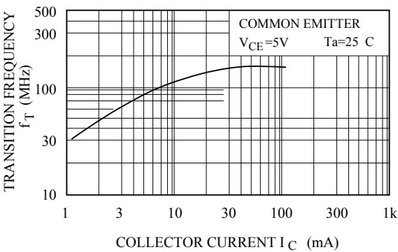
Current Gain-Bandwidth Product
