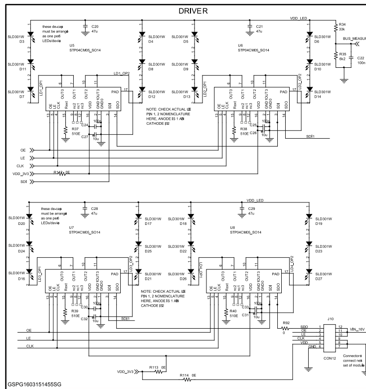
Figure 6: STEVAL-ILL071V1 circuit schematic (6 of 6)
