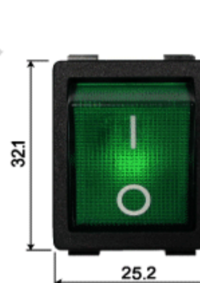
MOUNTING HOLE : 22 x 30mm
