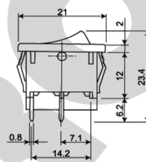
MOUNTING HOLE : 22 x 19.4mm
