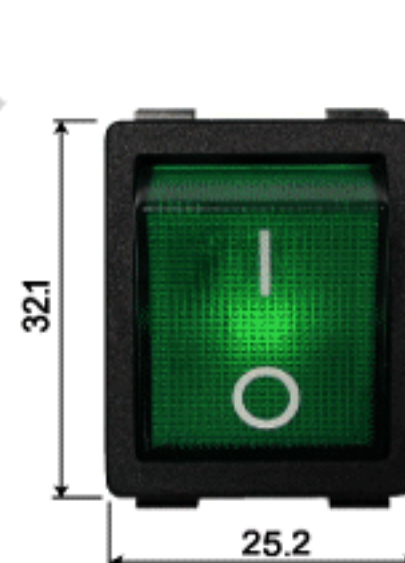
MOUNTING HOLE : 22 x 30mm
