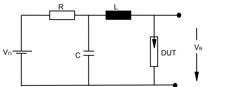
Fig. 3: QC- test circuit (sampling inspection at 25 °C)
