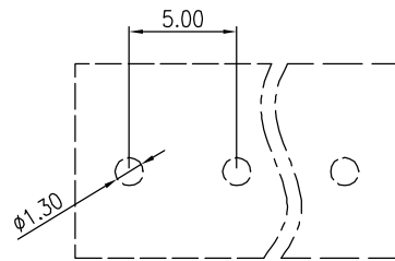
TOP VIEW-LAYOUT
