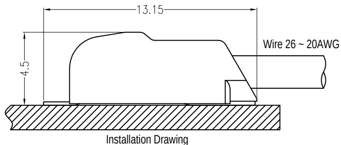
Installation Drawing
