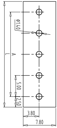
PCB LAYOUT S=2:1
