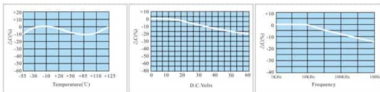
X7R/X5R Typical Characteristics
