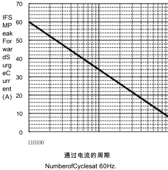
PEAK FORWARD SURGE CURRENT
