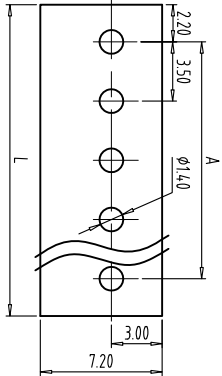
PCB LAYOUT S=3:1
